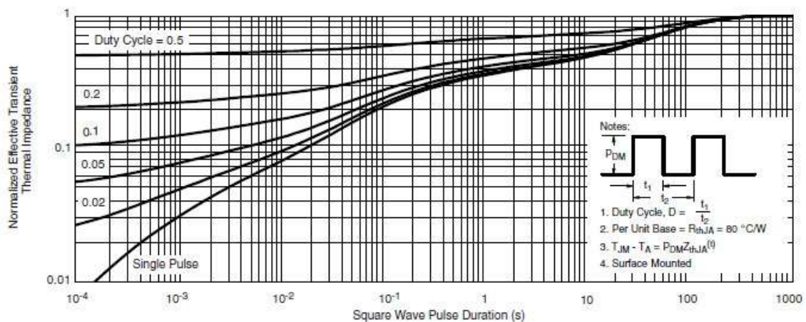
Normalized Thermal Transient Impedance, Junction-to-Ambient normalized thermal transient impedance, junction-to-foot
